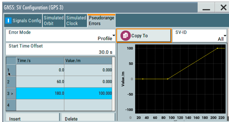
Simulation of a pseudorange ramp for SV 3 with the R&S®SMBV100B for testing the RAIM capabilities of a GNSS receiver
