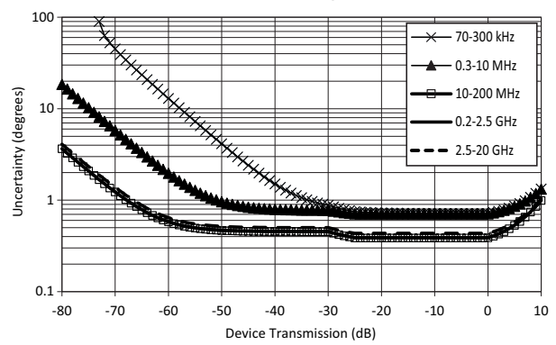
Transmission Phase Uncertainty; MS4642B (Opt. 8/9); 12-term Calibration using 36585K AutoCal
