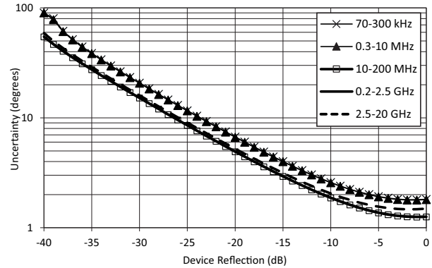
Reflection Phase Uncertainty; MS4642B (Opt. 8/9); SOLT-SL Calibration using 3650A-1 3.5 mm Cal Kit
