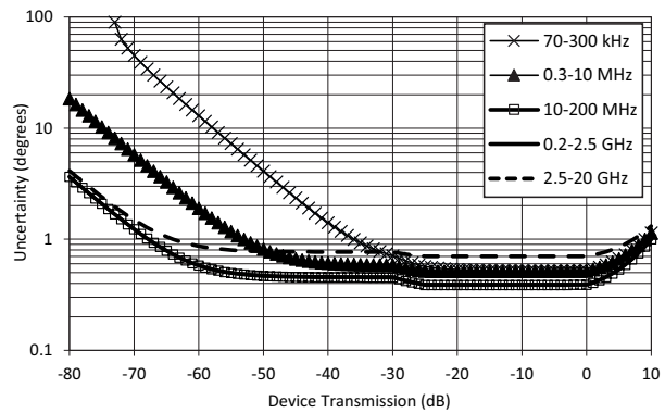
Transmission Phase Uncertainty; MS4642B (Opt. 8/9); SOLT-SL Calibration using 3650A-1 3.5 mm Cal Kit
