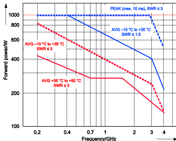
Power-handling capacity.
