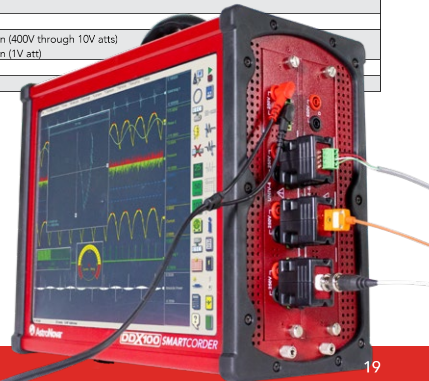
Different inputs with a single module
