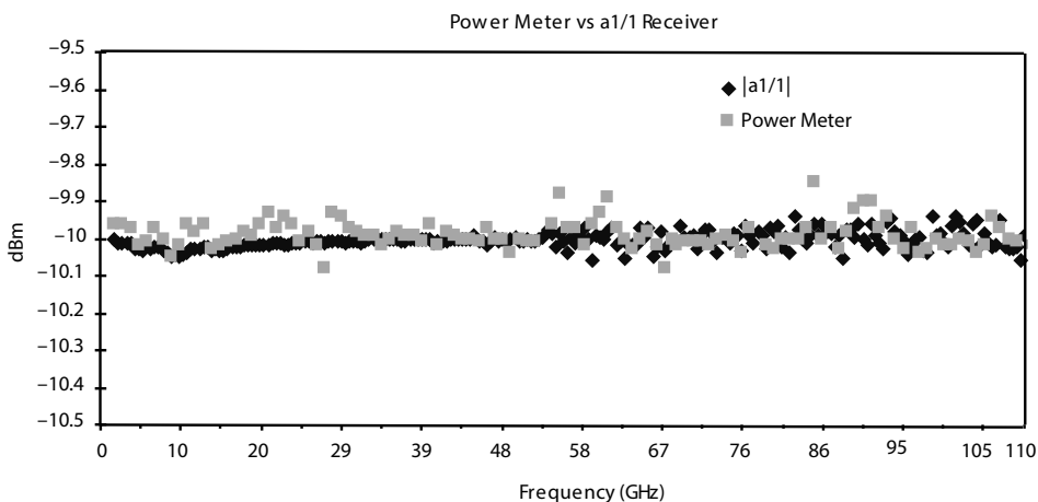
An example of typical power measurement agreement: power sensor vs. ME7838E a1 reference receiver.
