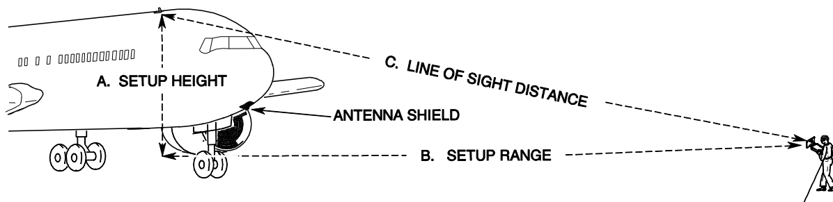
TESTING TOP ANTENNA
