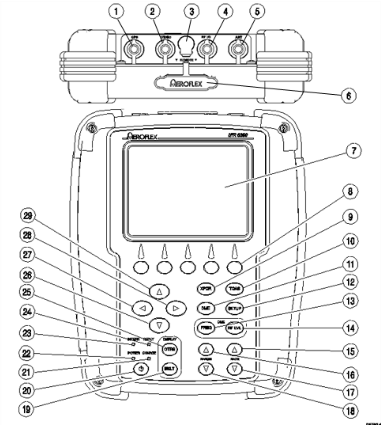
IFR 6000 Front Panel Figure 1
