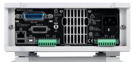
R&S®NGM202, rear view
