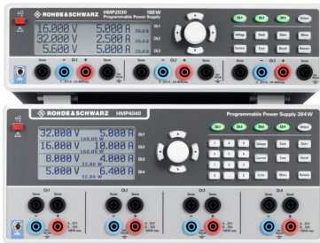
R&S®HMP2030 three-channel and R&S®HMP4040 four-channel power supply
