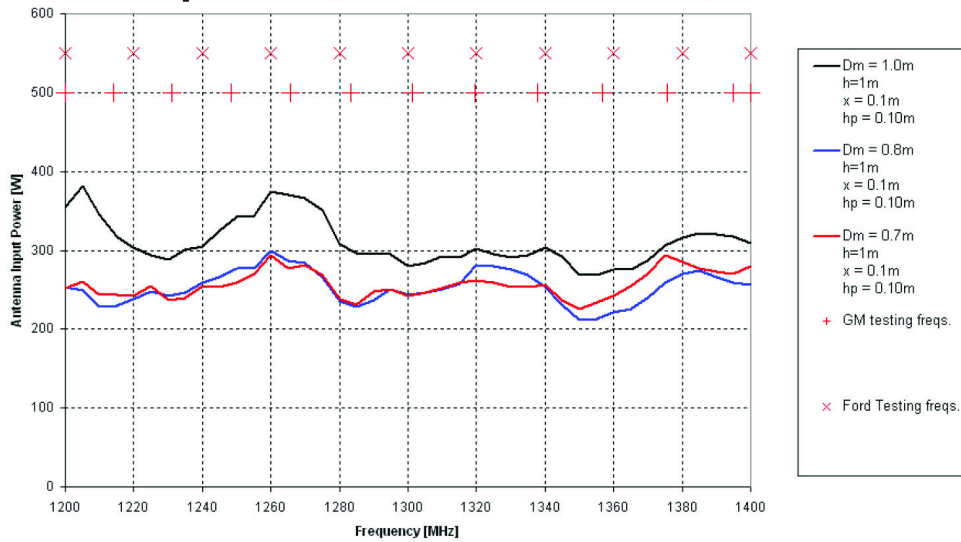
Antenna Input Power, Horizontal Polarization, With Test Points
