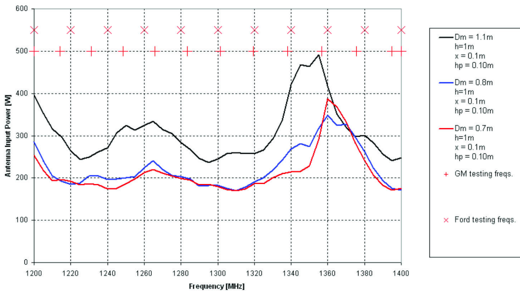
Antenna Input Power, Vertical Polarization, With Test Points
