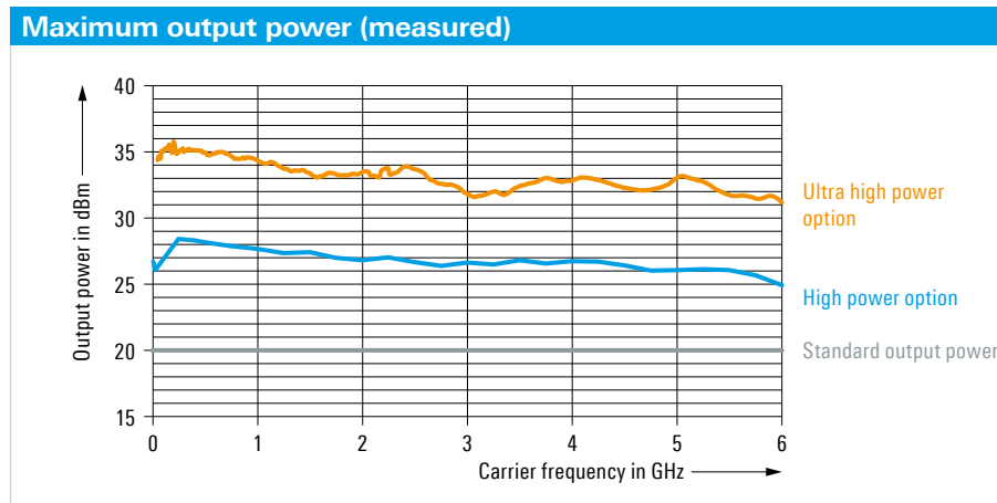
Measured output power for the base unit, with the high power option (R&S®SMBVB-K31) and with the additional ultra high power option (R&S®SMBVB-B32)
