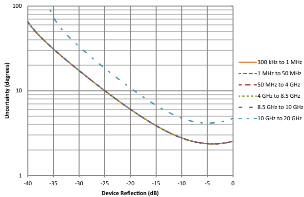
Return Loss Phase Uncertainty (degrees)
