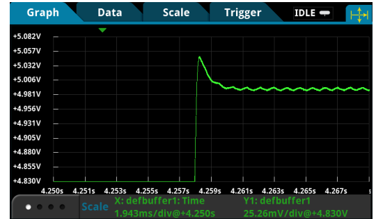
Analog measurement bandwidth
