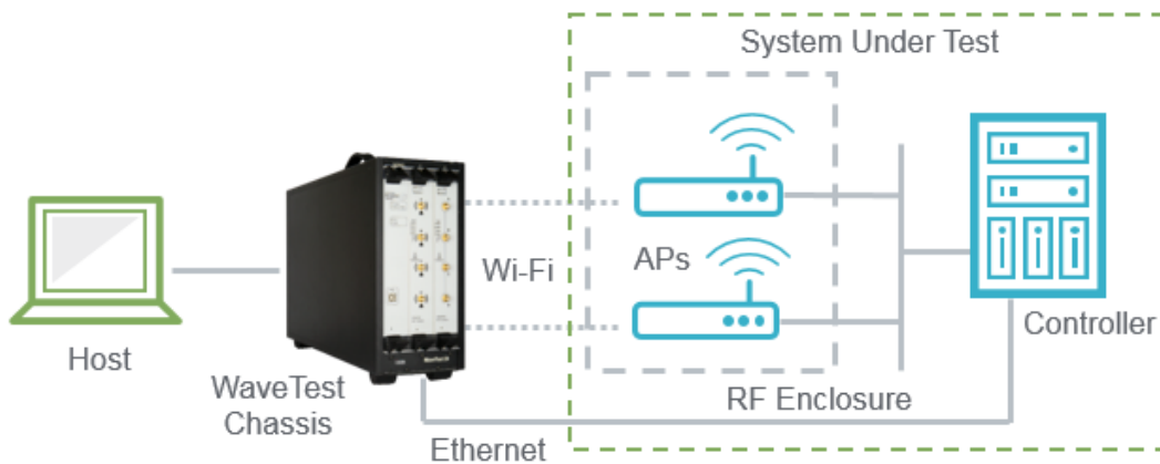
Wi-Fi Test Configuration
