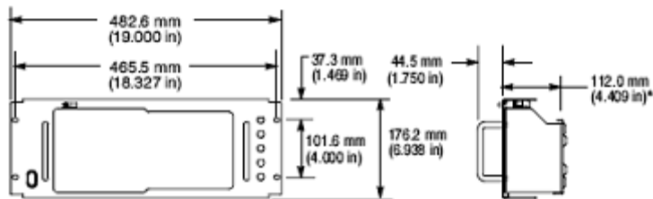
Figure 1: RM2000B Rackmount assembly
