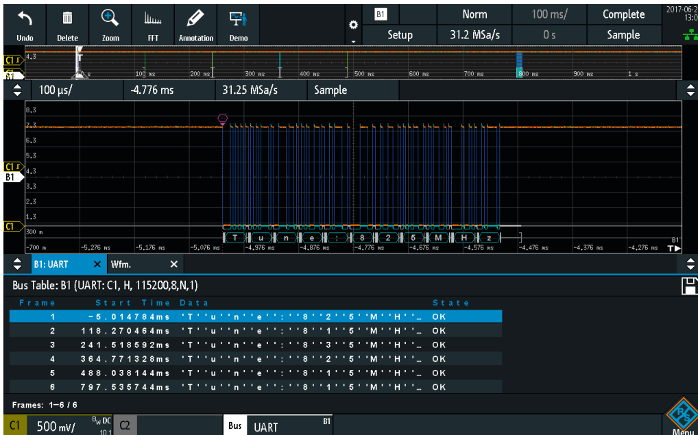
Decoded hexadecimal I 2 C message shown in honeycomb format and in table.
